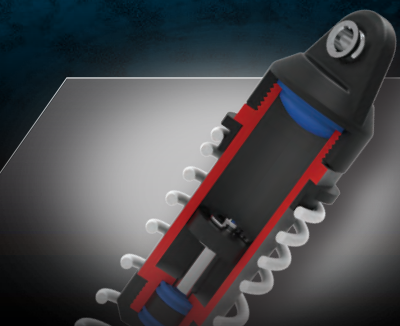
Oil-Filled Ultra Shocks™
